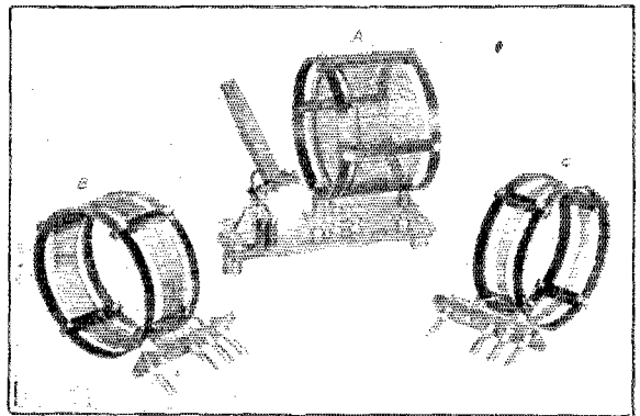
Fig. 2. The three "plug-in" coils and base holding adjustable primary. Note the small feedback coils inside of the main inductances. The coils here shown are made by Aero Products, Chicago.
