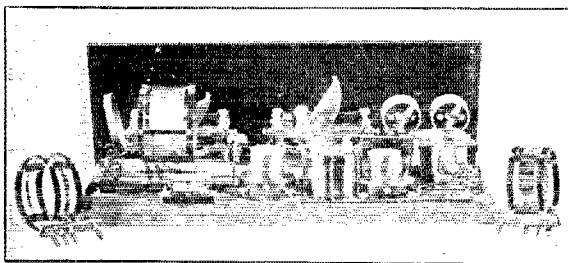
Fig. 3. Rear view of the receiver. Note plug-in grid leak and condenser and cushioned detector socket.
