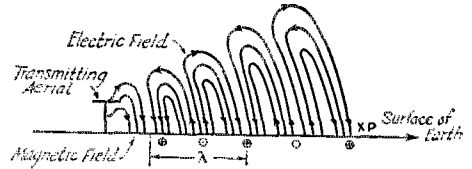
FIG. 2 THE FIELD RADIATING FROM AN ANTENNA WITH A GROUND CONNECTION.
